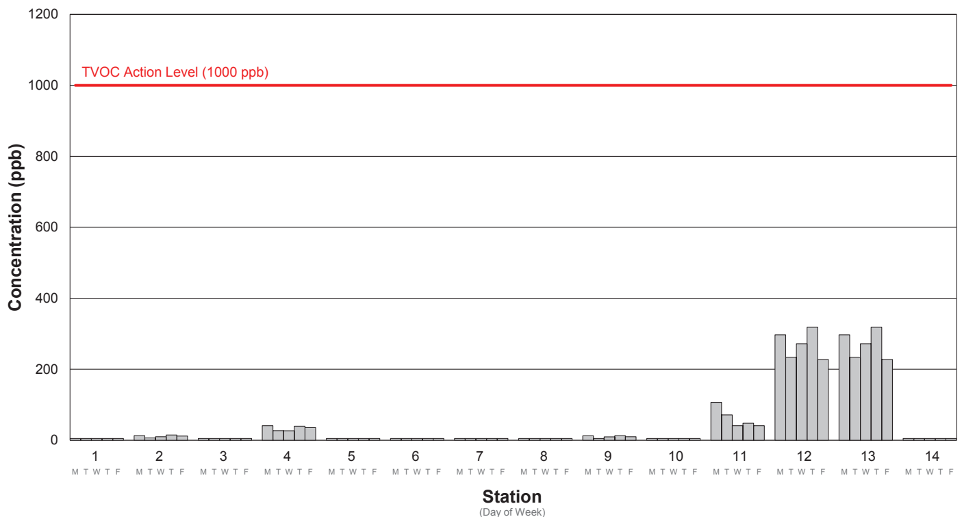
Average TVOC Concentration Week 47: 10/4/2021 - 10/8/2021
